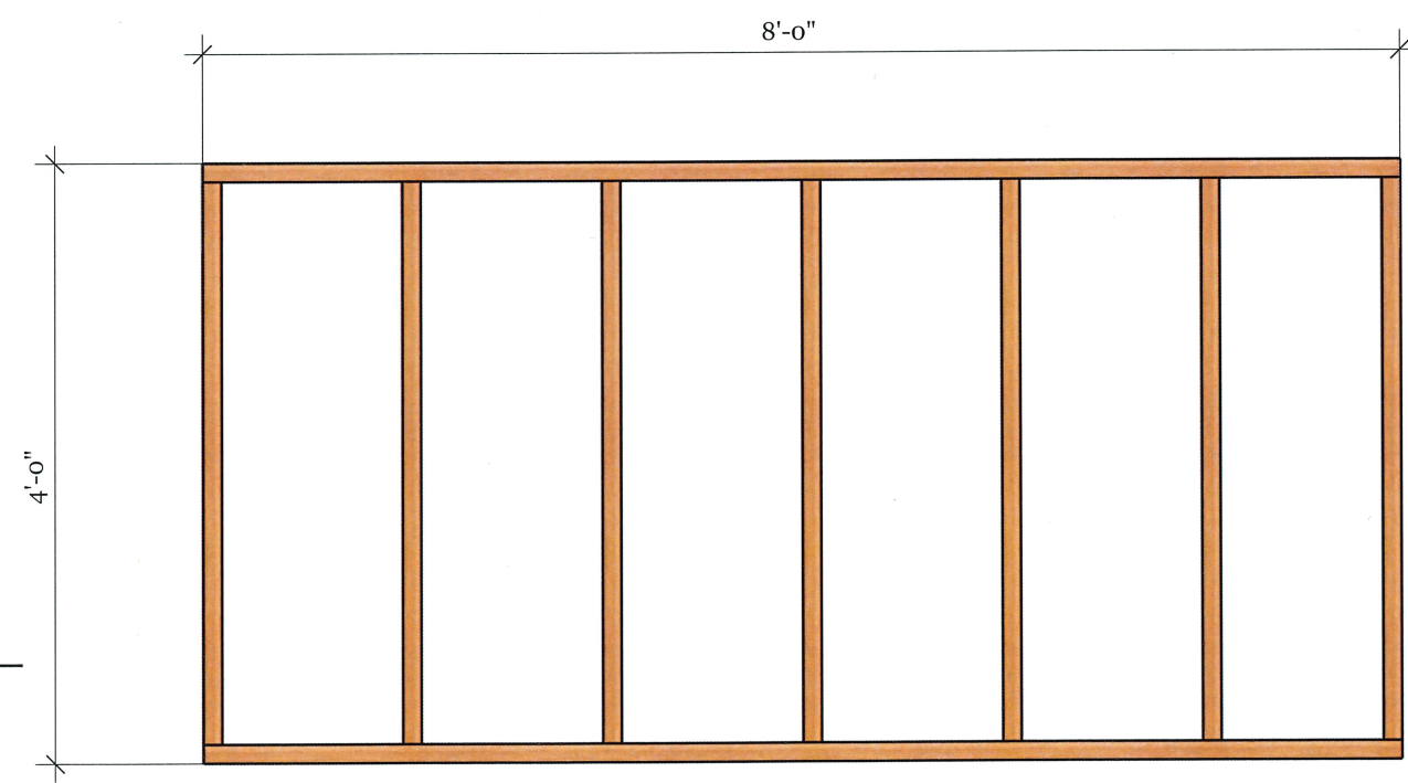
B Platform Plan @ 16"O/C A1 <Ratio>
